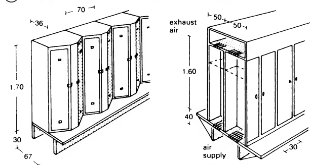
⑧ Trapezoid changing cubicles (Rotter system)
